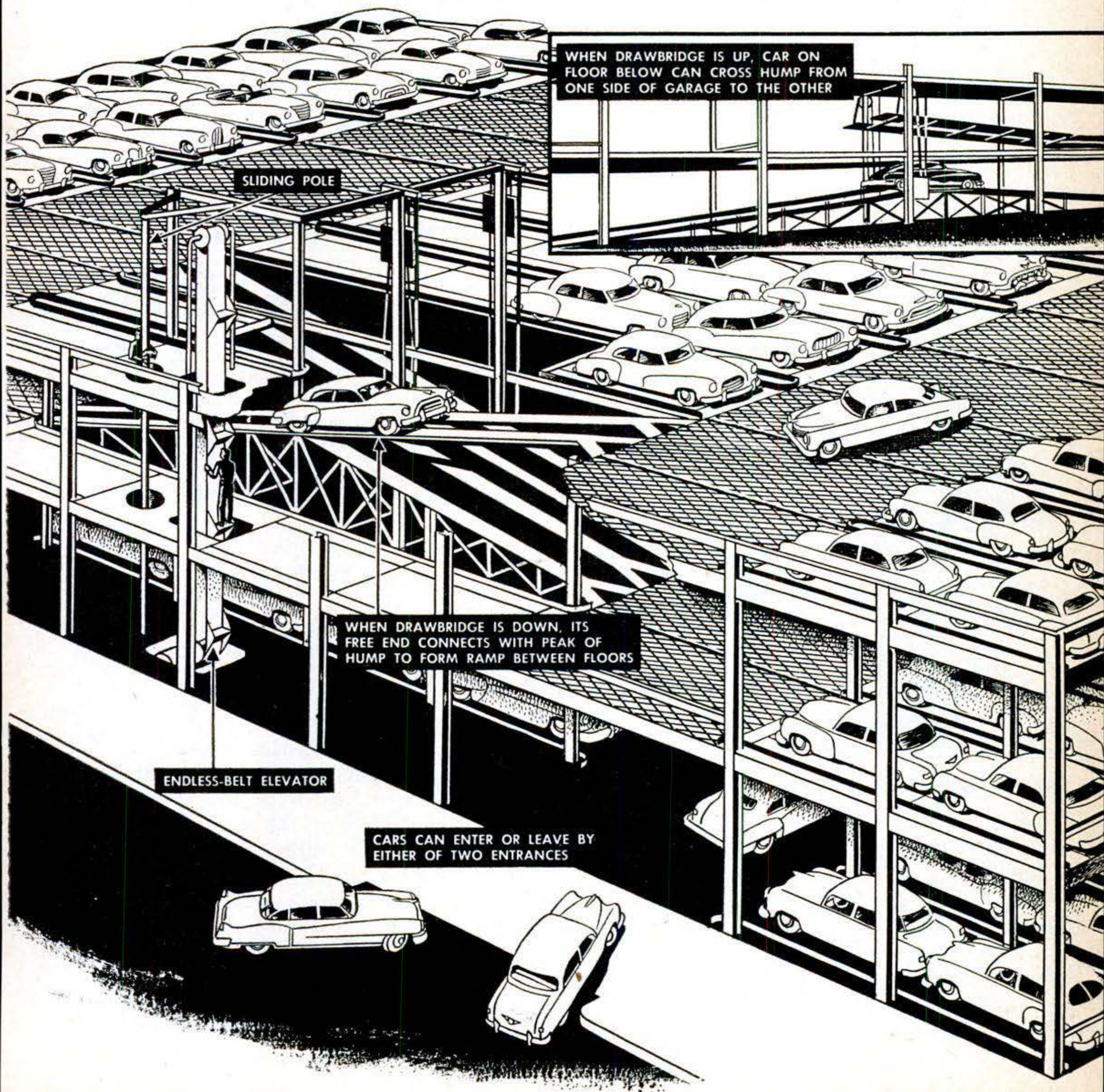
PUSH BUTTONS , operated by attendant from car, lower ramp to connect floors or raise it to let him drive across bridge on same floor.
